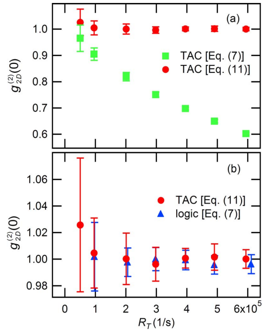
Fig. 4. (Color online) The degree of second-order coherence measured with two detectors g_{2D}^{(2)}(0) is plotted versus the singles rate on detector T , R_T . The sources of error are described in the text. In (a) data taken using the TAC is compared for analysis using Eqs. (7) and (11). In (b) data acquired using the TAC and the corrected expression Eq. (11) is compared to data acquired using the logic circuit and the uncorrected expression Eq. (7).
