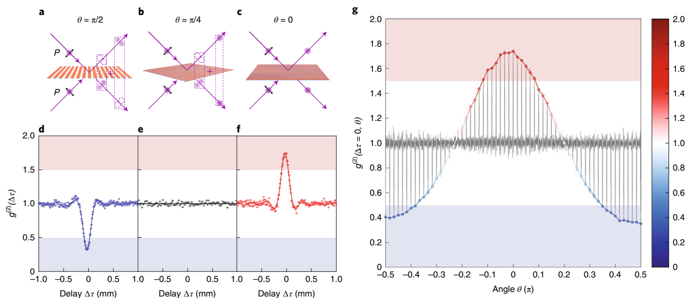
Fig. 2 | Experimental realization of the new DOF in the QTPI. a–c, Schematics of the distinct QTPI output states (as illustrated by the photons (solid purple balls) or no-photons (dotted purple circles) and associated dotted rectangles) at zero delay when the angle \theta is equal to \pi/2 , \pi/4 and 0, respectively, corresponding to the postselected bunching state (maximally entangled) and bosonic interaction (a), one of the intermediate states (partially entangled) and anyon-like interaction (b) and the antibunching state (totally disentangled) and fermion-like interaction (c). d–f, The measured g^{(2)}(\Delta\tau) between the two identical input photons in HOM-type coincidence measurements for the three cases in (a–c). The circles in (d–f) are the measured data with error bars (smaller than the circles) calculated assuming the Poisson distribution of event detection, and the solid curves are their fits. g, The measured g^{(2)}(\Delta\tau = 0, \theta) as a function of the rotation angle \theta enabled by the new DOF, simulating the continuous transition of effective quantum photon-photon interaction from bosonic bunching to fermionic antibunching. The open circle data points (coloured according to the colour bar) are extracted from 61 individual g^{(2)}(\Delta\tau, \theta) curves at each \theta value (the catenated grey curves). In d–g , the fitted g^{(2)}(\Delta\tau = 0) values have an uncertainty of \pm 0.03 at the 95% confidence level and the shaded areas mark the regions arising from the pure quantum effect.
