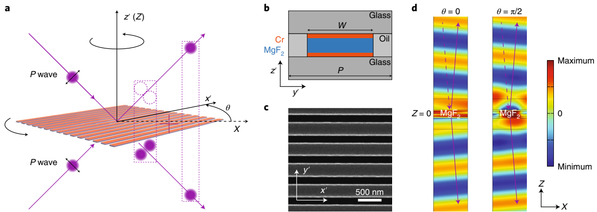
Fig. 1 | Introduction of a new DOF in optical quantum interference by a non-unitary metasurface. a , Given the polarization of the input photons (solid purple balls), for example, P waves, the rotational DOF at the metasurface along its surface normal ( z' axis) creates a new synthetic DOF in QTPI. The emergent DOF is specified by the angle \theta between the metasurface local x' axis (along the strips) and the laboratory X axis (along the intersection line between the incident plane and the metasurface). The output of QTPI and the associated effective quantum photon–photon interaction can be controlled by changing \theta , as illustrated by a superposition of states (solid purple balls) or no-photons (dotted purple circles). b , The metasurface unit structure consists of a three-layer strip made of Cr/MgF 2 /Cr (18/59/18 nm) in the z' direction, with 240 nm width ( W ) and 395 nm period ( P ) in the y' direction. The strip is sandwiched by two glass plates with index-matching oil filling the gap. c , Top-view scanning helium-ion microscope image of the metasurface (typically 36 \mu\text{m} \times 36 \mu\text{m} ). d , The simulated transmitted and reflected magnetic fields' y component ( H_y , colour bar) around the metasurface. The reflection plot in Z > 0 space is derived by subtracting the incident field from the total field. Arrows indicate the propagation directions.
