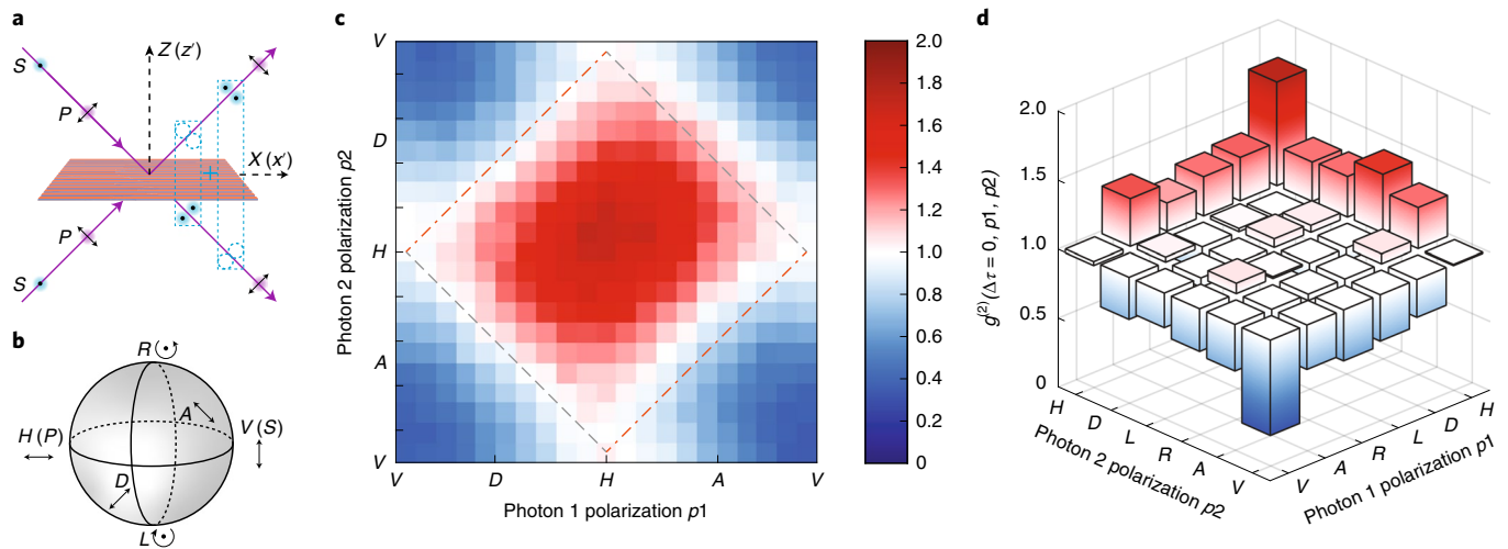
Fig. 3 | The generalized QTPI for independent photon polarizations. a , Schematics of the measurement where the metasurface is fixed at \theta=0 , while the polarization states of the two incident photons were regulated independently. The case with both photons polarized in P ( S ) wave is illustrated by purple (blue) balls or circles and associated dotted rectangles. b , The Bloch sphere representation of the polarization state where the P ( S ) wave is defined as the H ( V ) state. The six representative states H (horizontal), V (vertical), D (diagonal), A (anti-diagonal), L (left circular) and R (right circular) are labelled. c , The measured g^{(2)}(\Delta\tau=0, p_1, p_2) map as a function of the polarizations of the two photons, showing a rich texture and a continuous transition from bosonic bunching to fermionic antibunching. The white regions marked by grey dashed lines correspond to no interference when the two photons have orthogonal polarization, whereas the white regions marked by red dash-dot lines correspond to a balanced superposition of the two extreme eigen-operation interferences. A small shift of the white regions with respect to the dashed lines is due to the imperfection of wave plates. d , The measured g^{(2)}(\Delta\tau=0, p_1, p_2) values with the two photons in the six representative states H , V , D , A , L and R . In c–d , the fitted g^{(2)}(\Delta\tau=0) values have an uncertainty of \pm 0.03 at the 95% confidence level.
